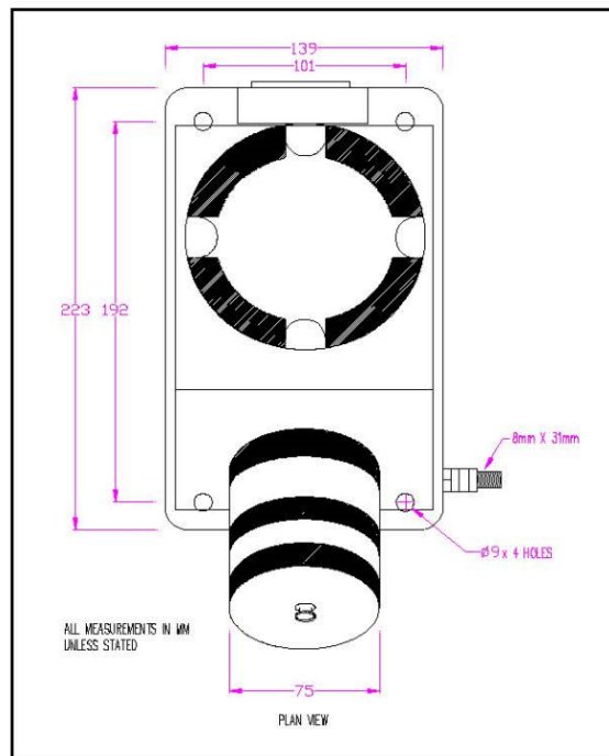
PYLE Connector Plan View
