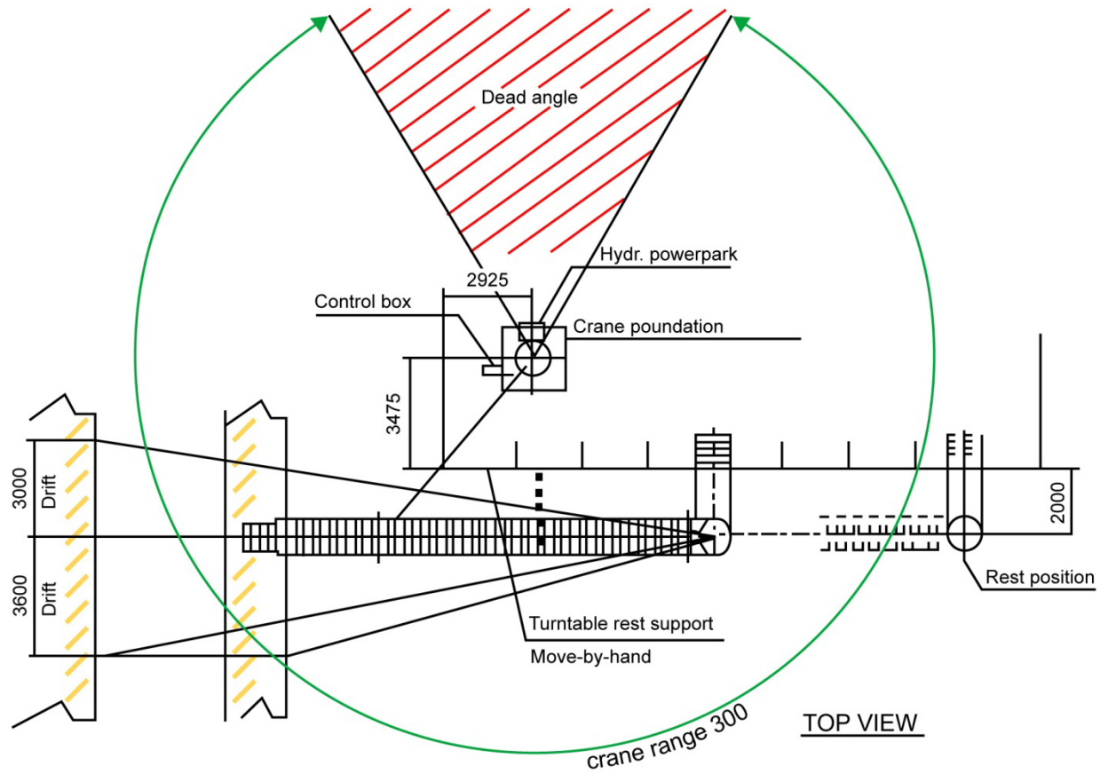
Figure 8-8 Gangway Plan
