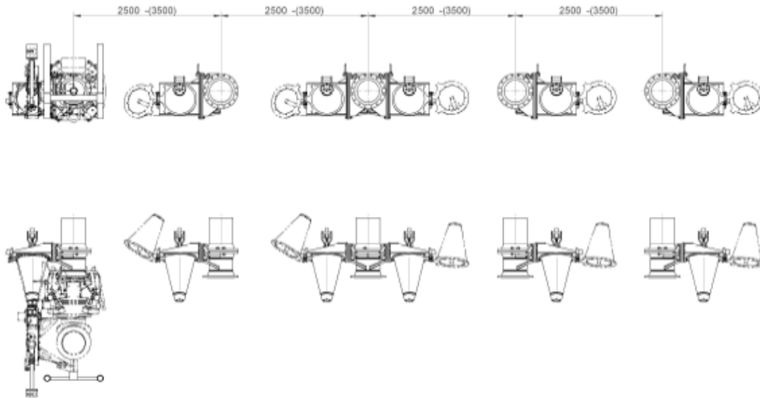
Figure 8-6 Typical Configuration with Spools at LNGC Manifolds
