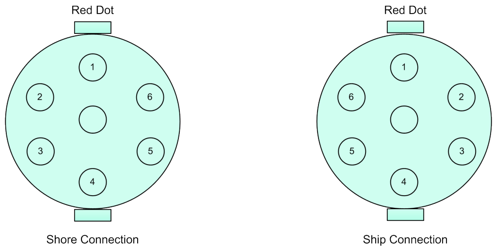
Figure 8-10 Pin-out Configuration
