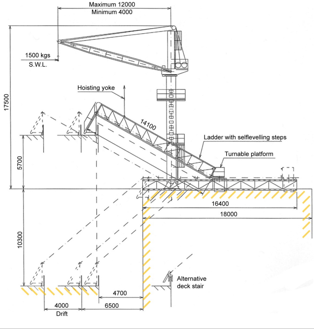
Figure 8-7 Gangway Profile
