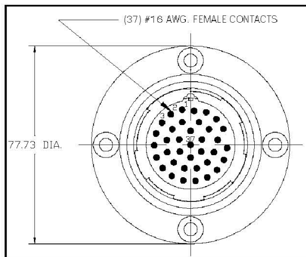
PYLE Connector Pinout
