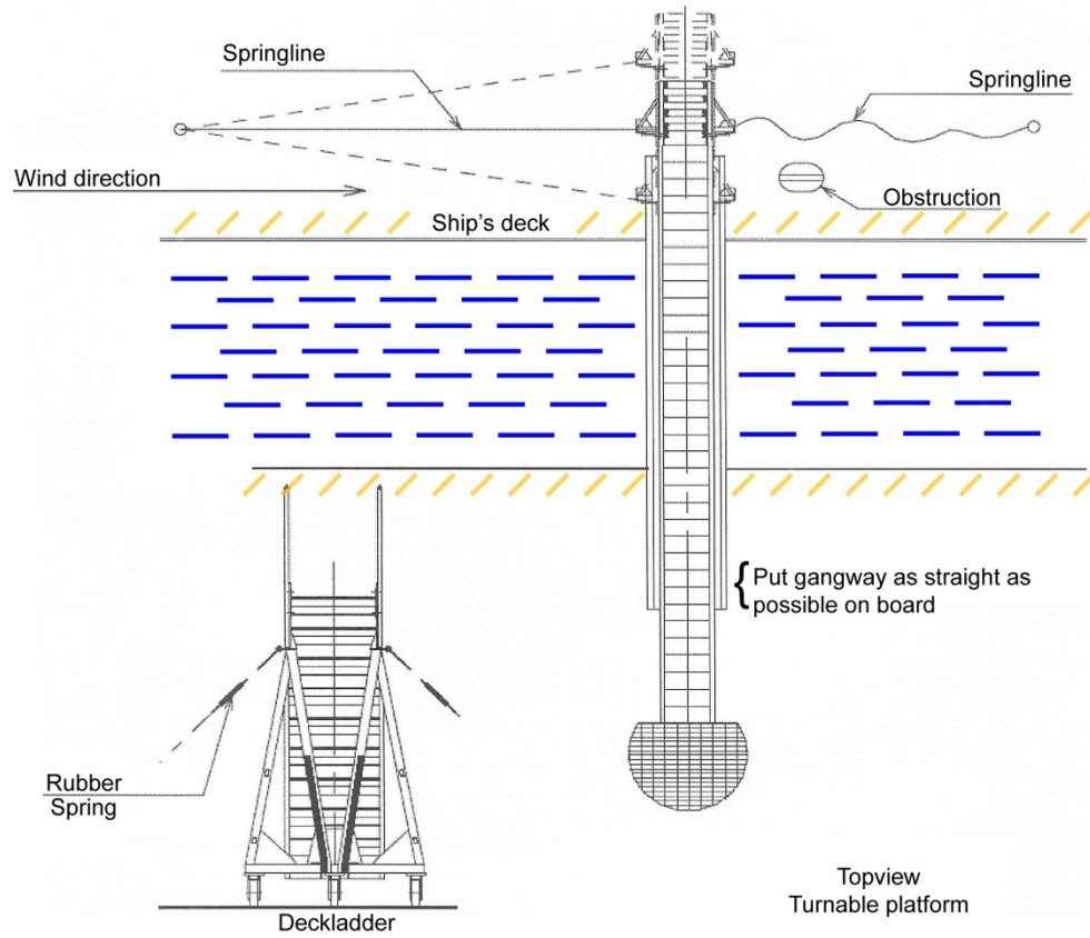
Figure 8-9 Gangway Spring Arrangements
