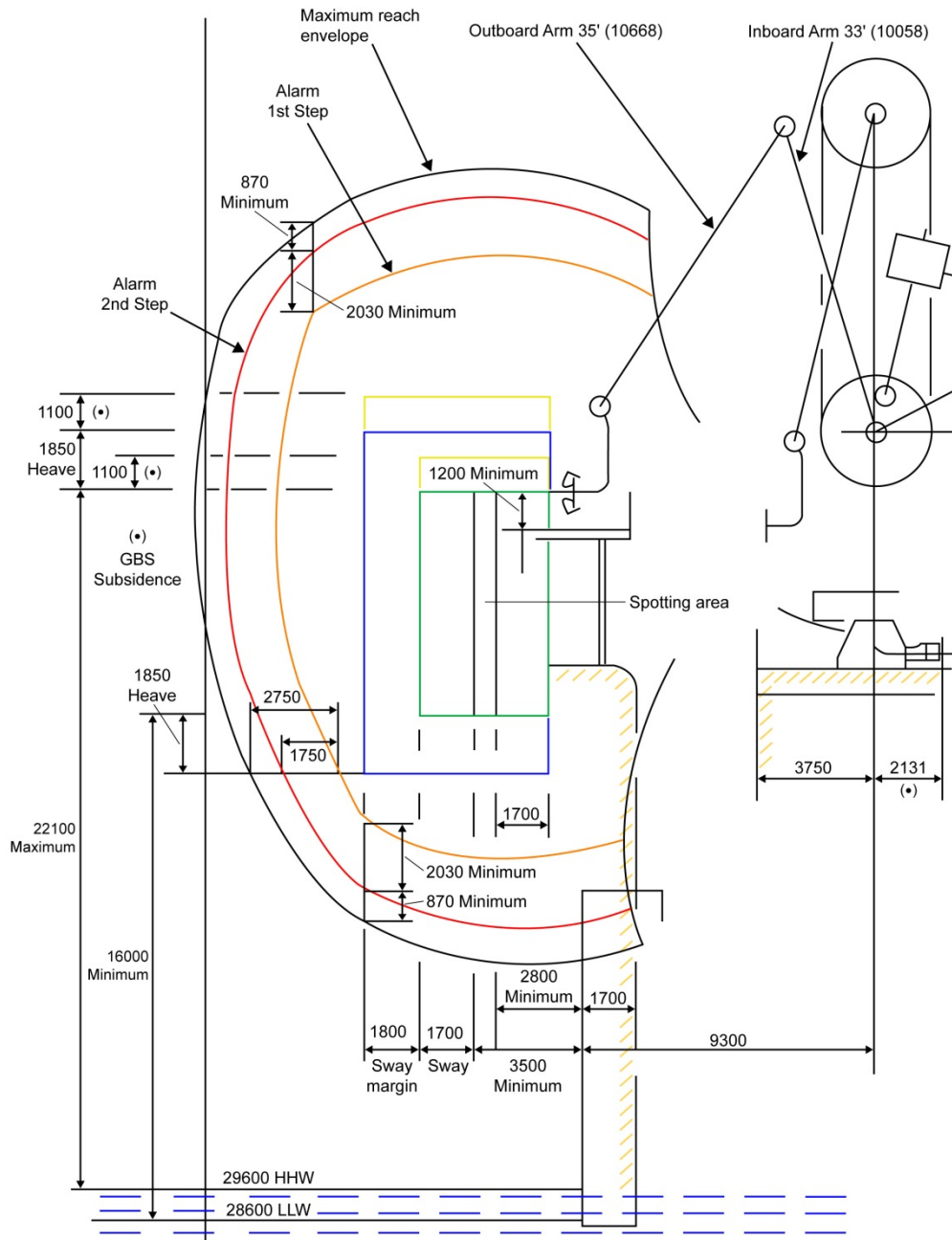
Figure 8-3 Loading Arm Envelope – Elevation
