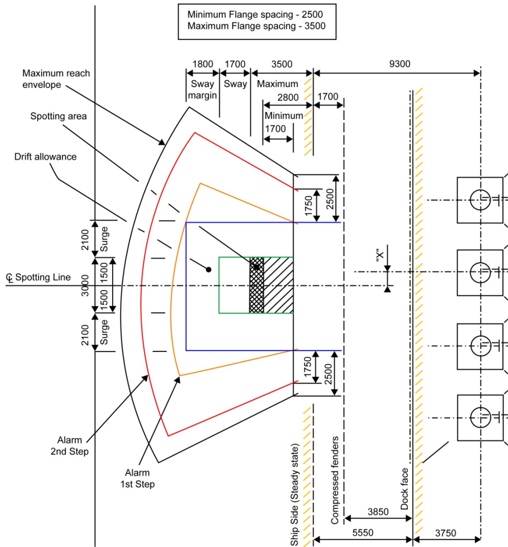
Figure 8-2 Loading Arm Envelopes – Plan
