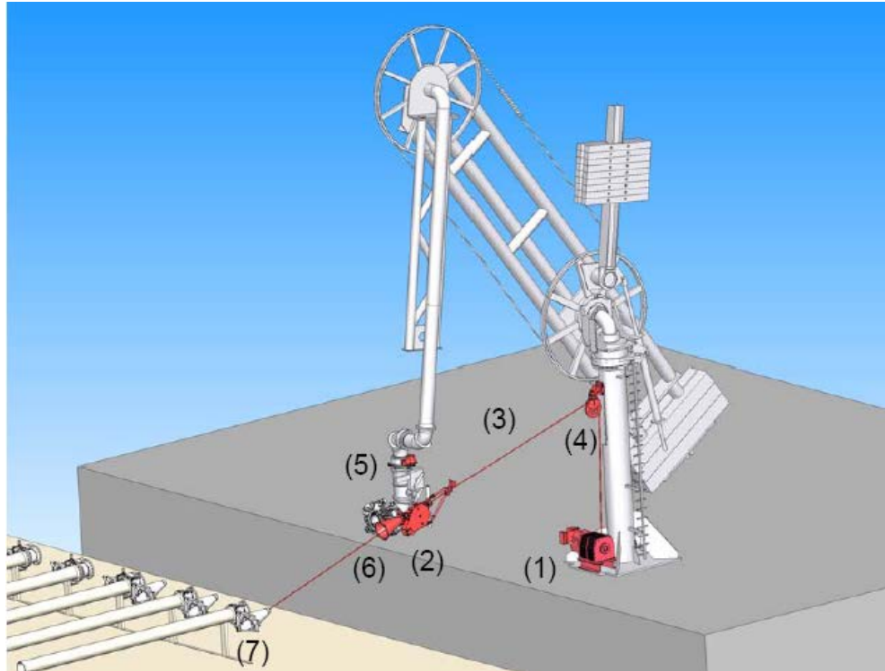
Figure 8-5 Loading Arm and Major Components
