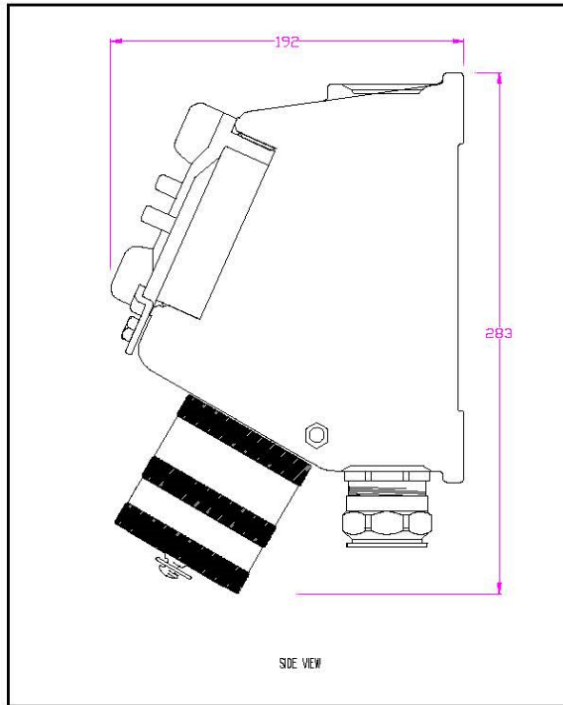
PYLE Connector Side View
